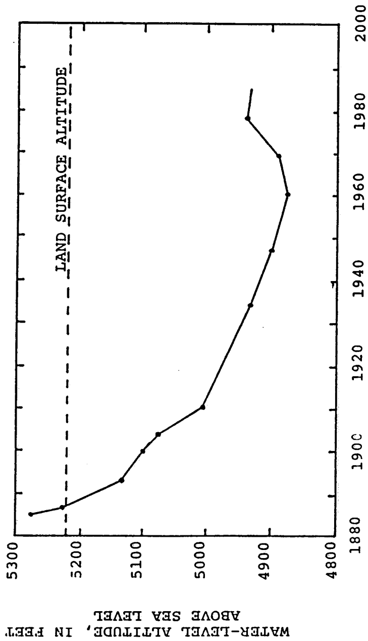
Figure 6. Water-level hydrograph for the Arapahoe aquifer near the Colorado Capital Building (Robson, 1984).
