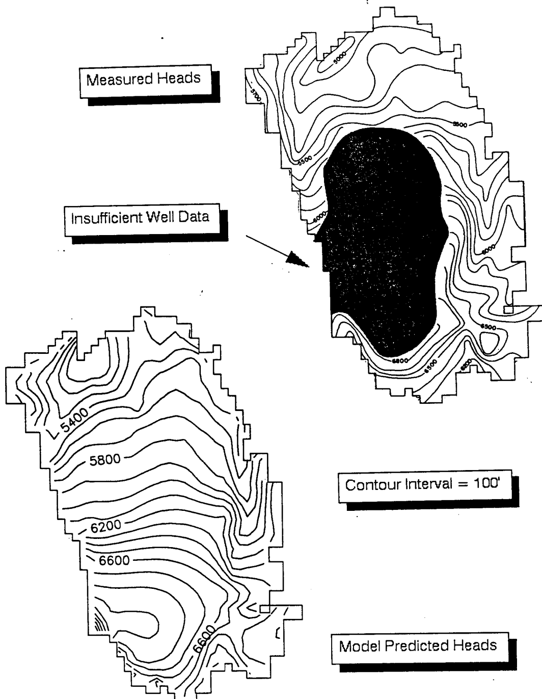
Figure 7. Comparison of measured and model predicted 1978 potentiometric surface of the Denver aquifer (Location of the aquifer is given in Fig. 4)
