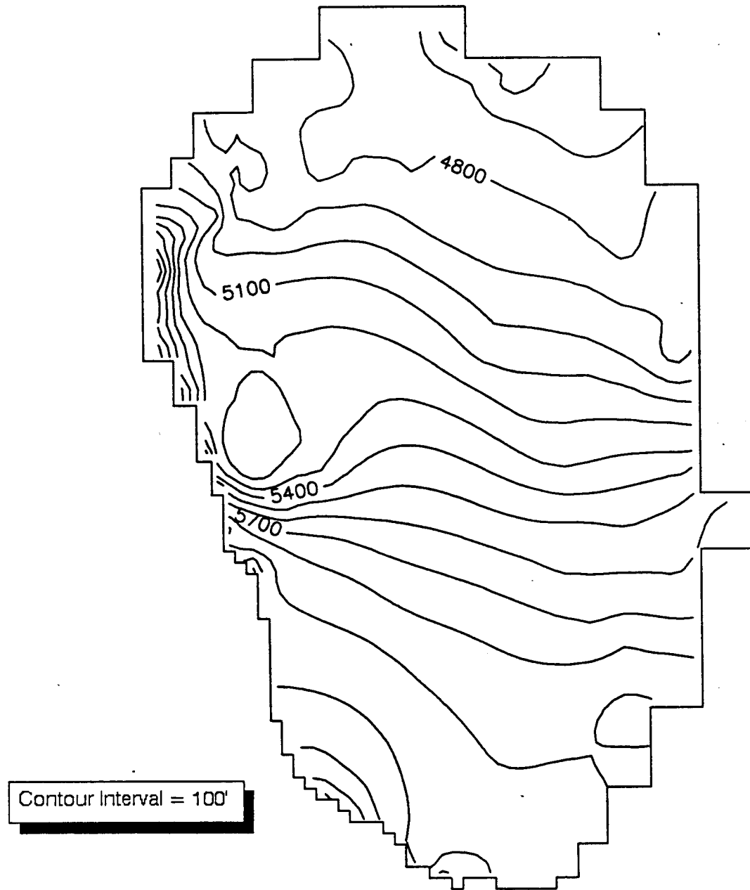
Figure 10. Model predicted 1978 potentiometric surface of the Laramie-Fox Hills aquifer (Location of the aquifer is given in Fig. 4)
