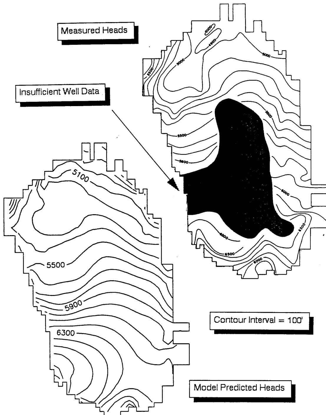
Figure 8. Comparison of measured and model predicted 1978 potentiometric surface of the Arapahoe aquifer (Location of the aquifer is given in Fig. 4)
