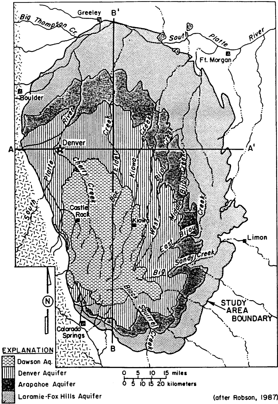
Figure 2. The four principal aquifers in the Denver Basin (after Schenk and Poeter, 1990)
