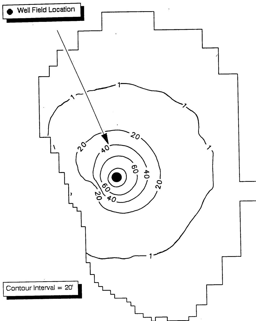
Figure 26. Water level decline in the Laramie-Fox Hills aquifer after the 3rd drought period in DAPS2 (Location of the aquifer is given in Fig. 4)
