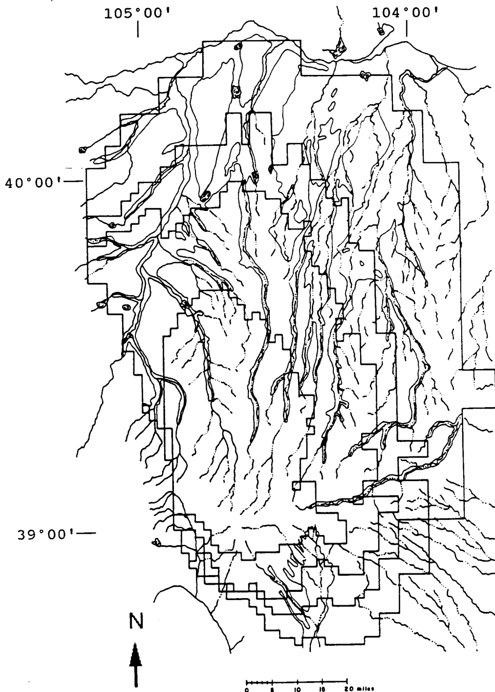
Figure 5. Drainages of the Denver Basin with outlined bedrock aquifers (after Schenk and Poeter, 1990)
