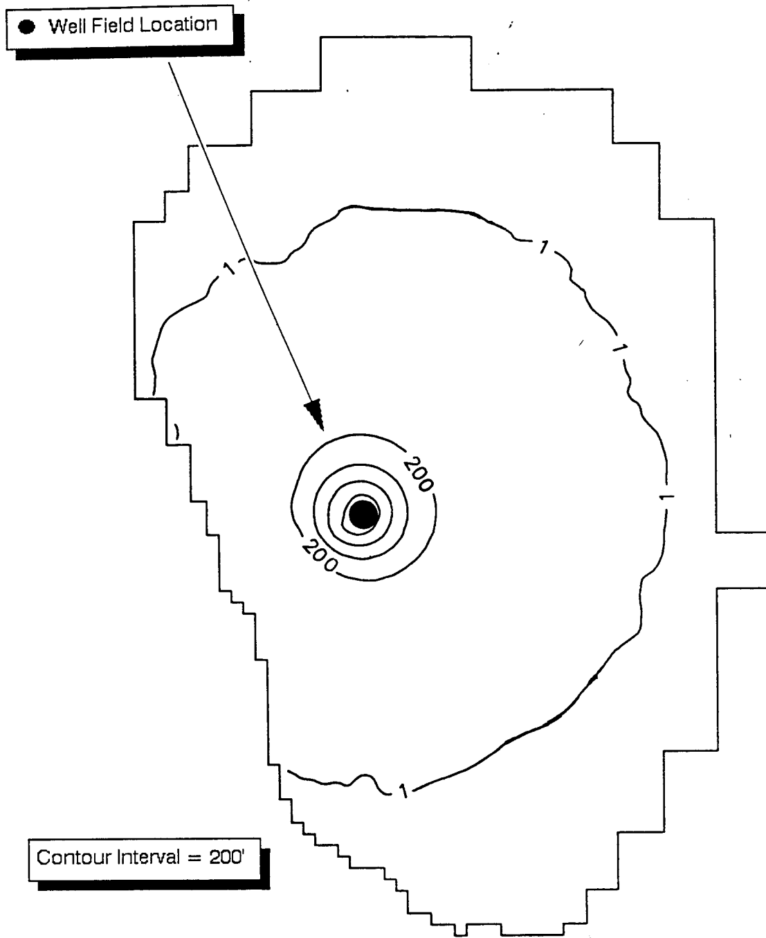
Figure 21. Water level decline in the Laramie-Fox Hills aquifer after the 6th drought period in DAPS1 (Location of the aquifer is given in Fig. 4)
