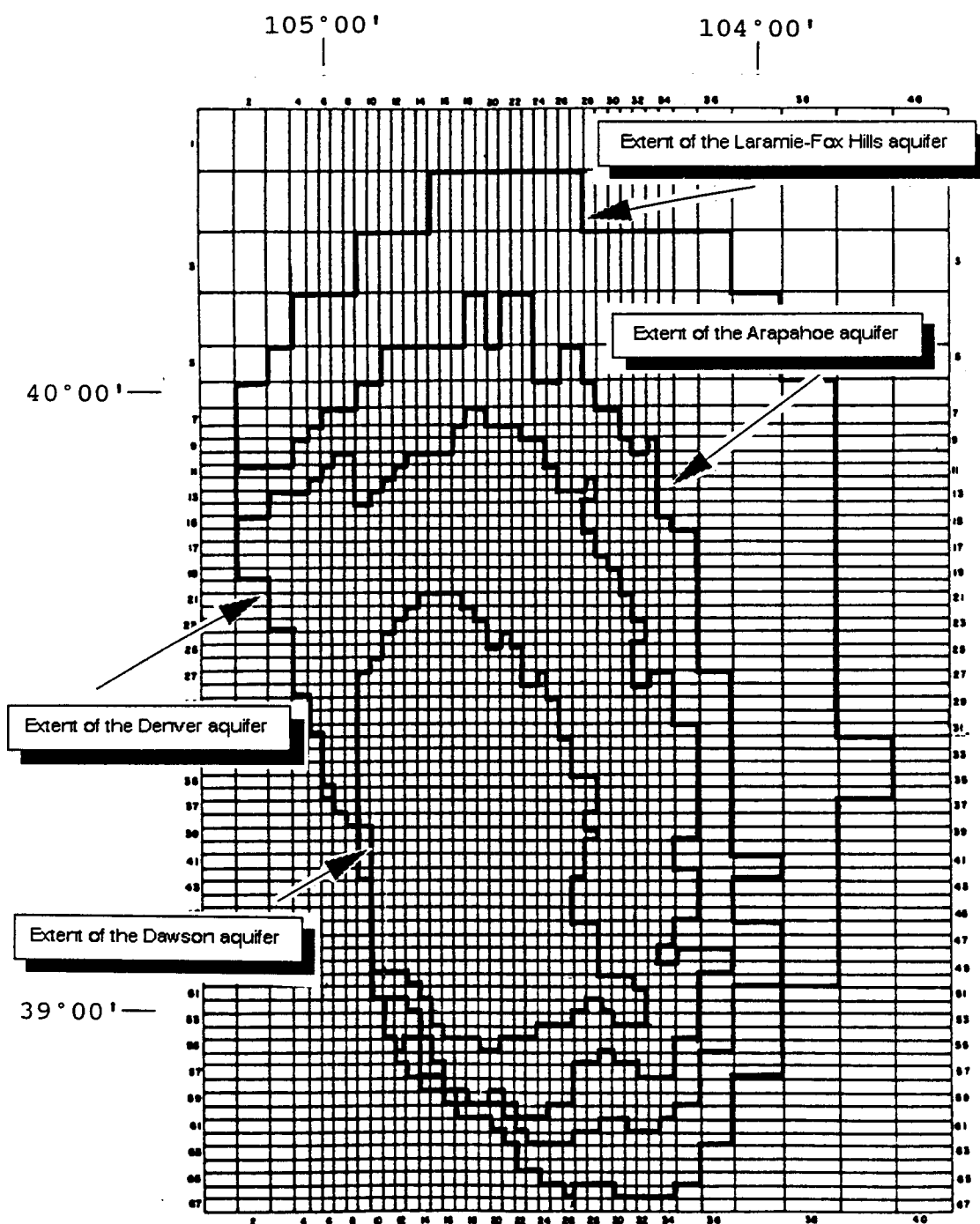
Figure 4. Finite difference grid with outlined Denver Basin bedrock aquifers (after Schenk and Poeter, 1990)
