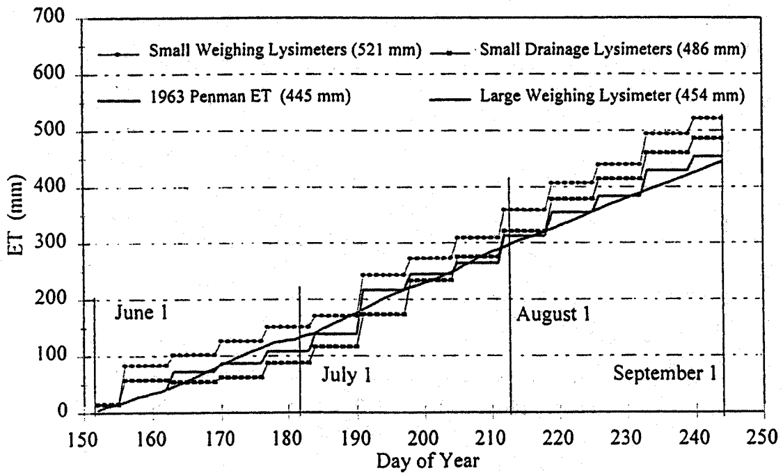
Fig. 9.d. Daily Cumulative ET Measured by Lysimeters and 1963 Penman - 1995 Season.
