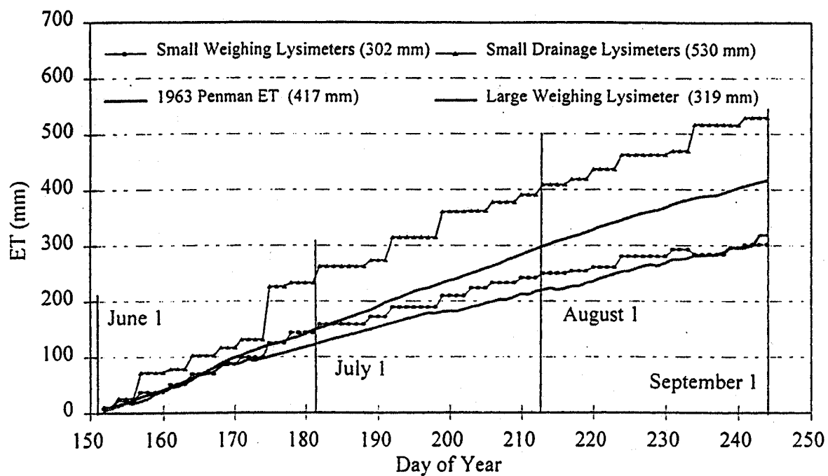
Fig. 9.b. Daily Cumulative ET Measured by Lysimeters and 1963 Penman - 1993 Season.
