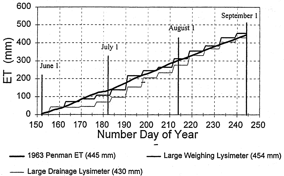
Fig. 8. ET Estimations by 1963 Penman and Large Weighing Lysimeter
