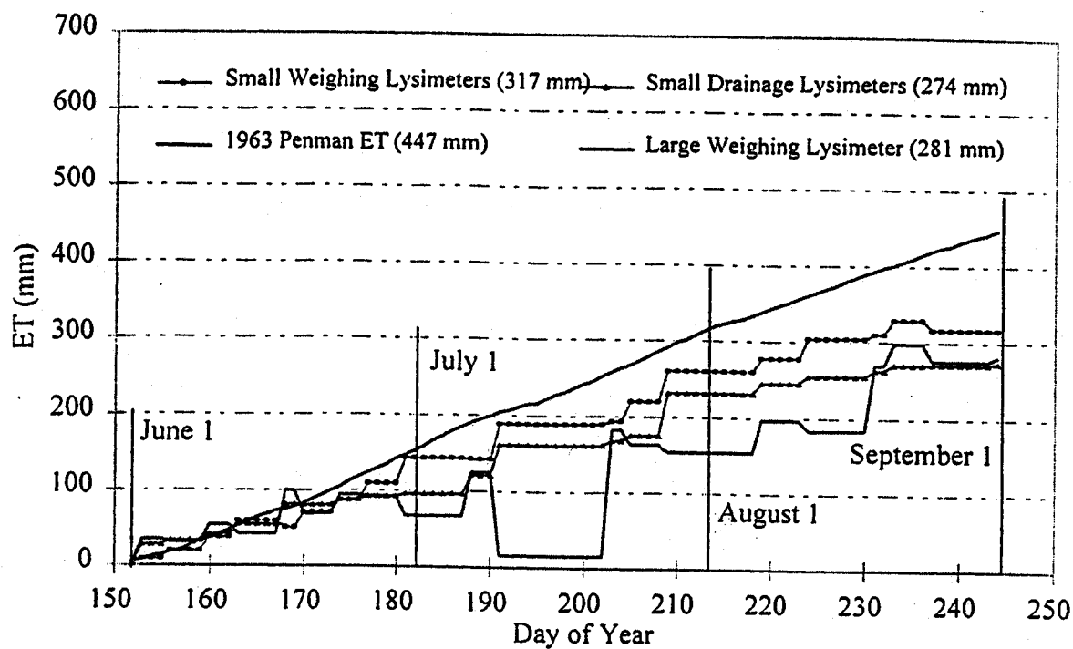
Fig. 9.a. Daily Cumulative ET Measured by Lysimeters and 1963 Penman - 1992 Season.
