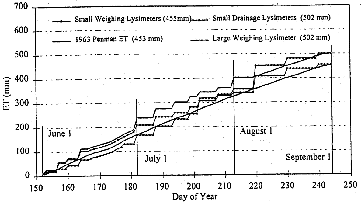
Fig. 9.c. Daily Cumulative ET Measured by Lysimeters and 1963 Penman - 1994 Season.
