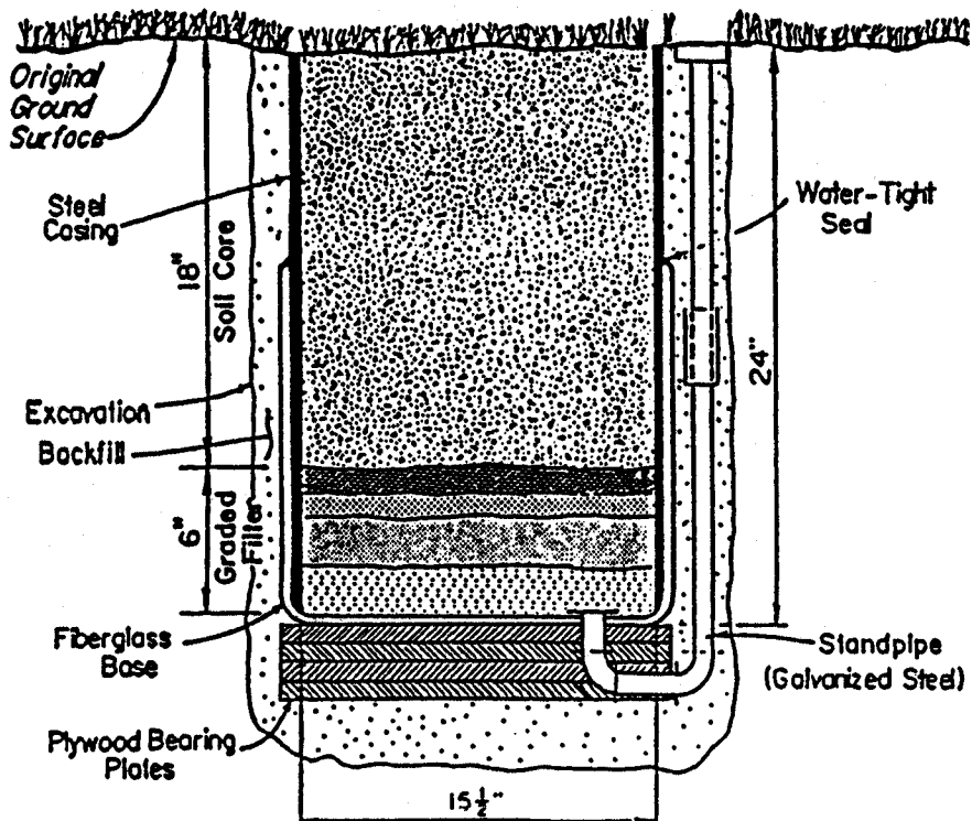
Fig. 4.b. Small Drainage-Type Lysimeter
