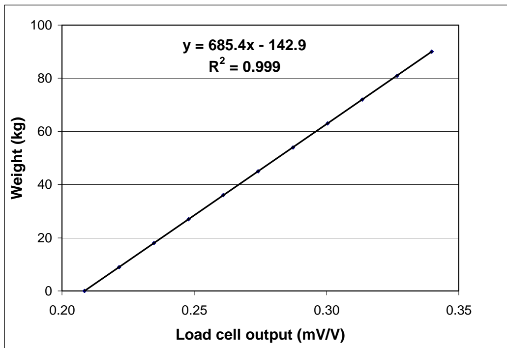
Figure 13. Weight as a function of load cell output Calibration data analyzed by Dale Straw of DWR
