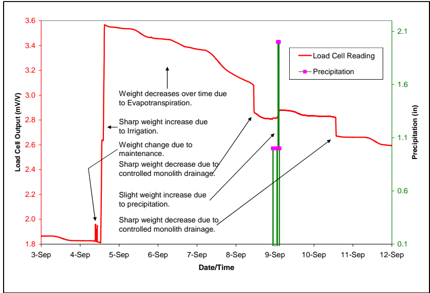
Figure 10. Load cell and precipitation readings for 3-12 September 2006 Graph by Lane Simmons
