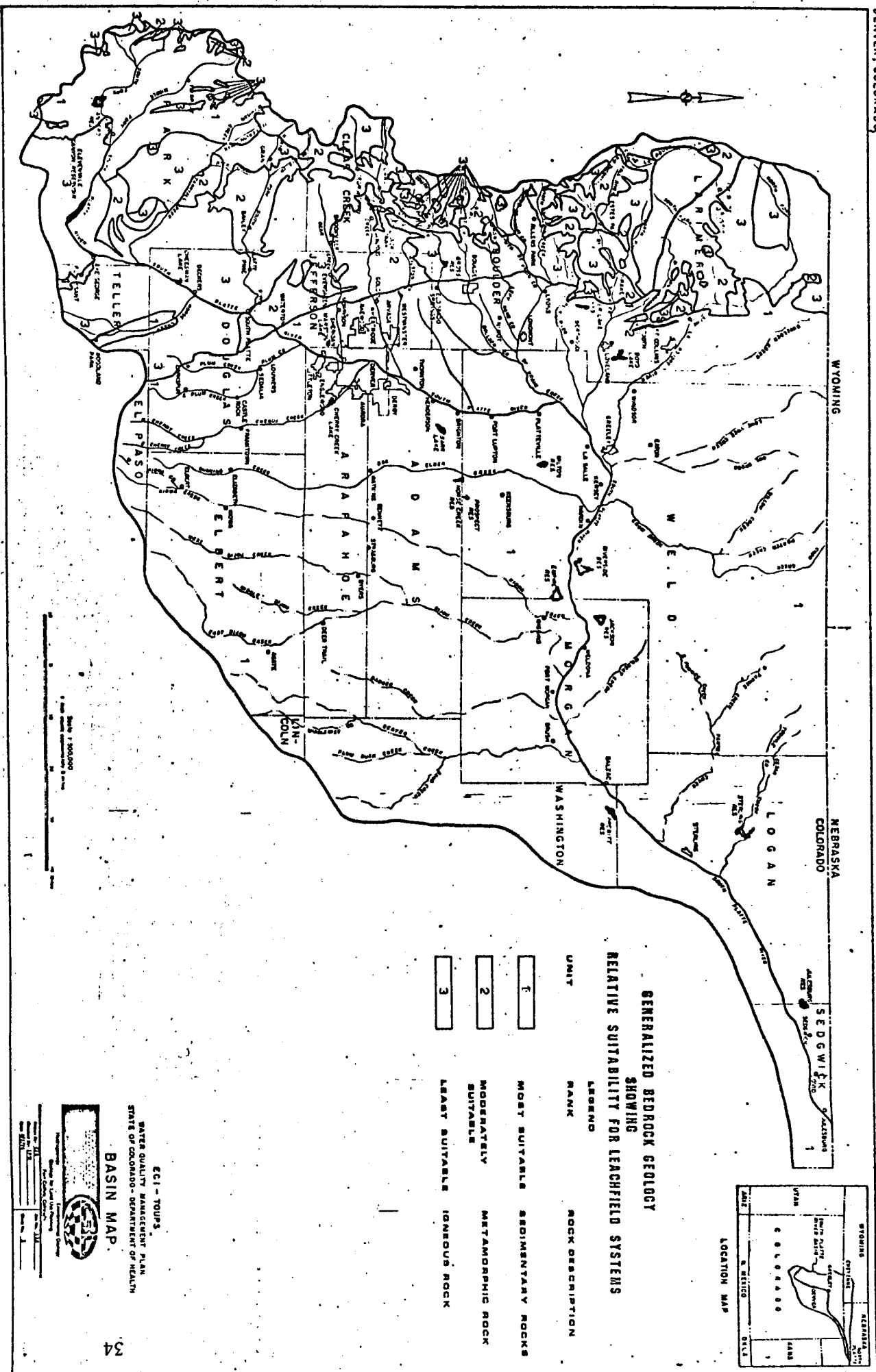
Plate 2. Generalized Bedrock Geology Map of the South Platte River Basin.
