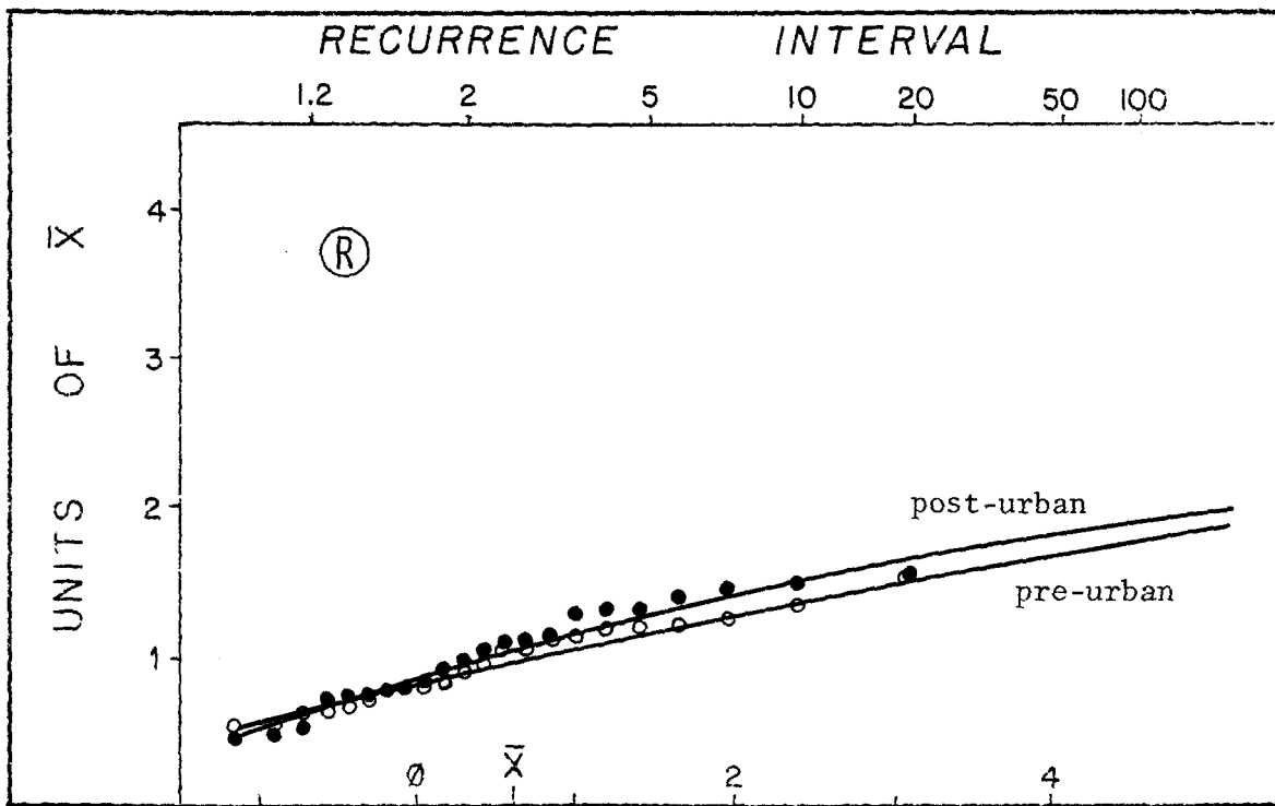
FIGURE 38. Flood frequency curves, Quinebaug River.
