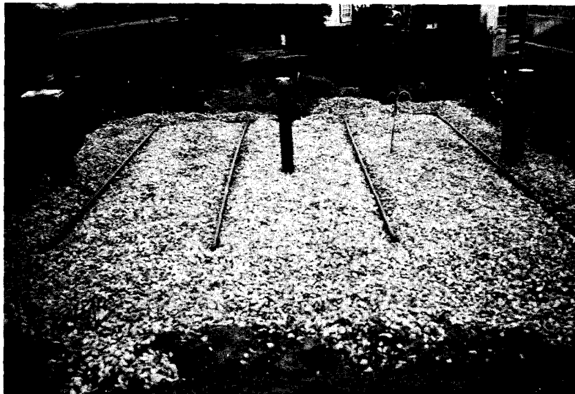
Fig. 8. Lay the distribution pipe on the stones, taking care to lay the laterals level. Slope the manifold slightly toward the inlet pipe. Remove dips and rises in laterals. Cover distribution system with 2 in. of stone. Do not drive on top of distribution system.
