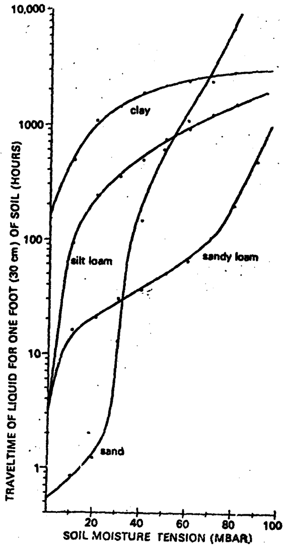
Figure I-B.2. Traveltime of Liquid for One Foot of Soil at Different Soil Moisture Tensions, Calculated for Four Soil Materials (Bouma et al. , 1972)
