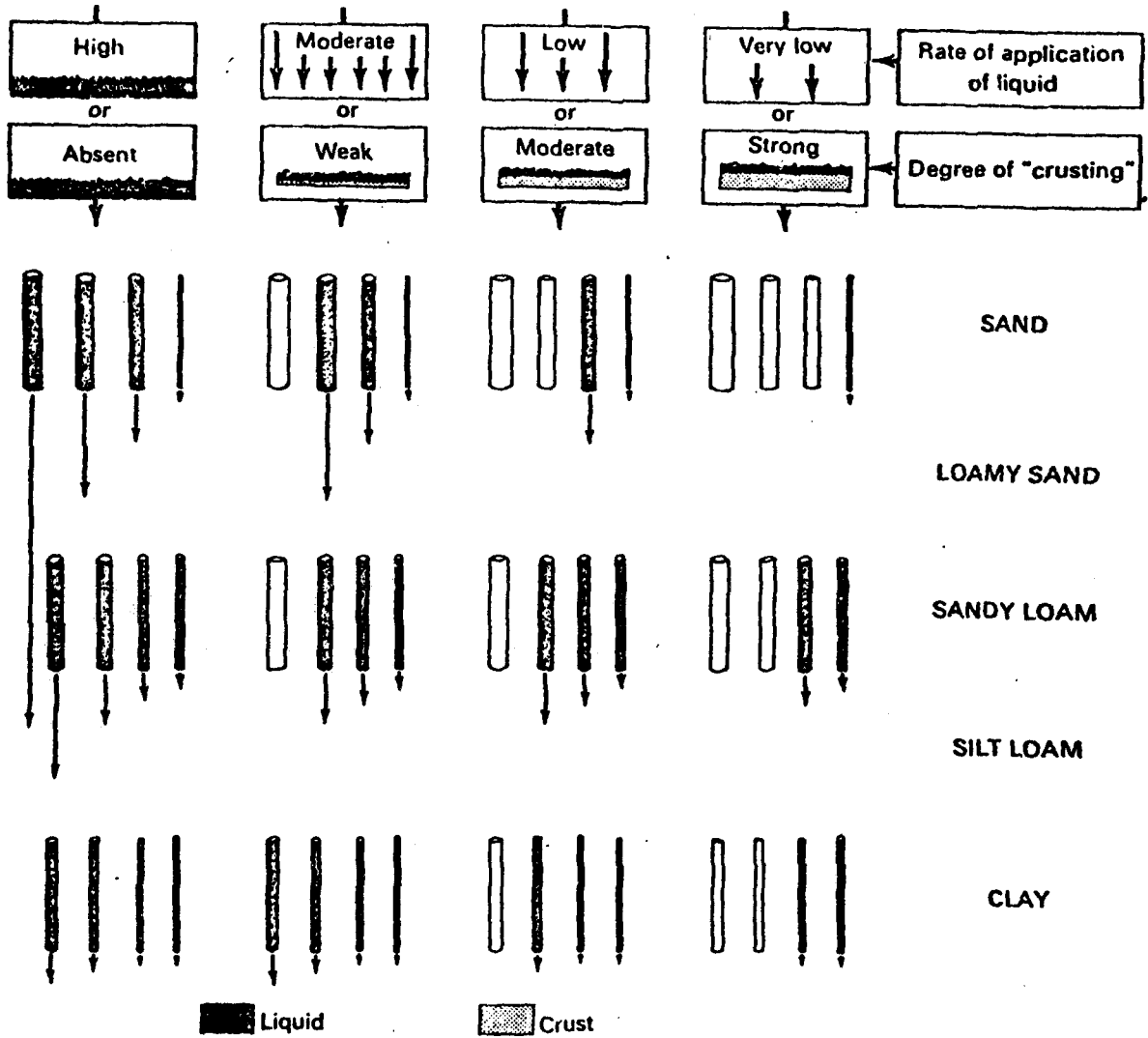
Figure I-A.3.a. Schematic Diagram Showing the Effect of Increasing the Degree of Crusting or Decreasing the Rate of Application of Liquid on the Rate of Percolation Through Three "Soil Materials," (Bouma et al. , 1972)
