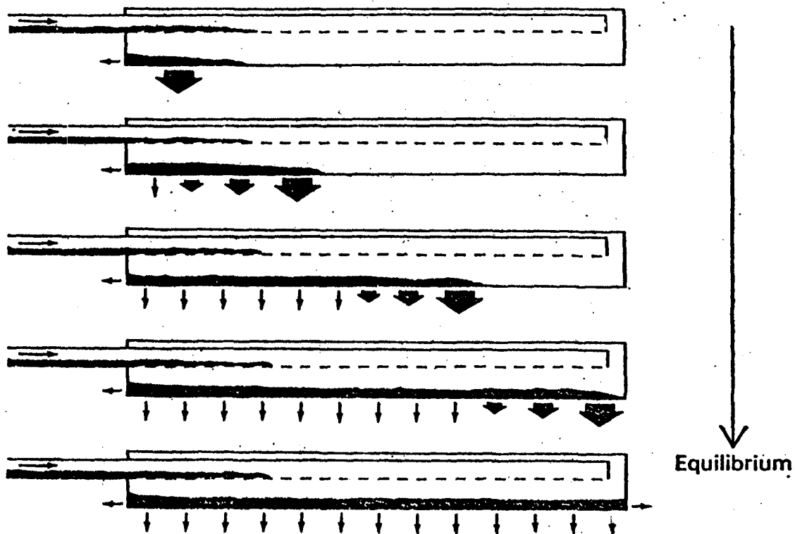
Figure I-B.1. Progressive Crusting of the Infiltrative Surfaces of Subsurface Seepage Beds. (Bouma et al. , 1972)
