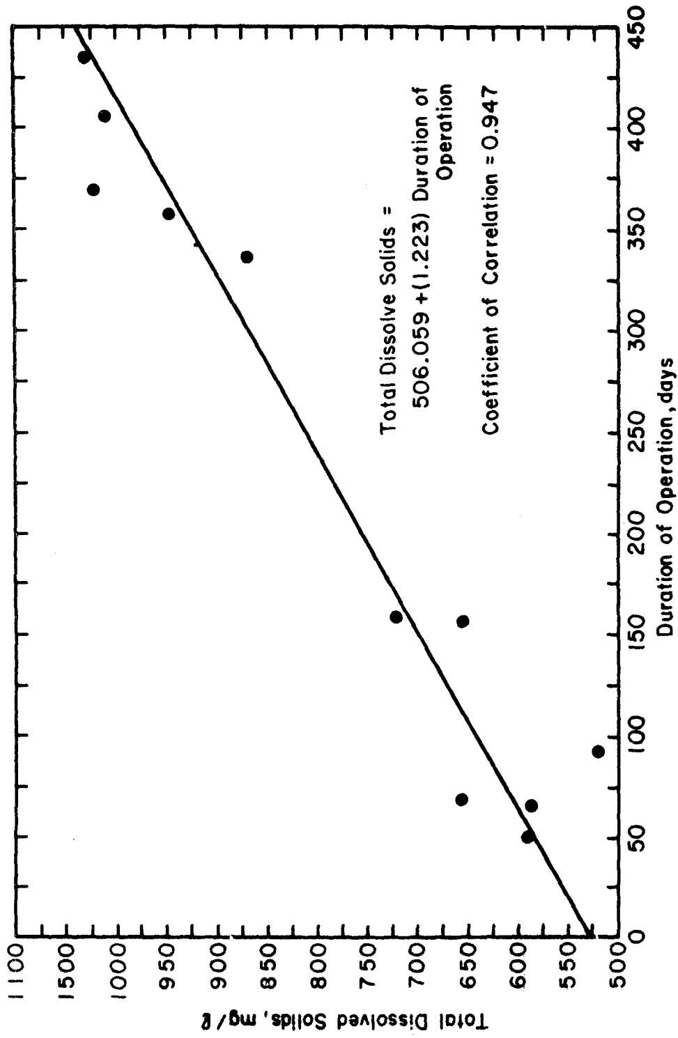
Figure VII-22. Total Dissolved Solids Versus Duration of Operations
