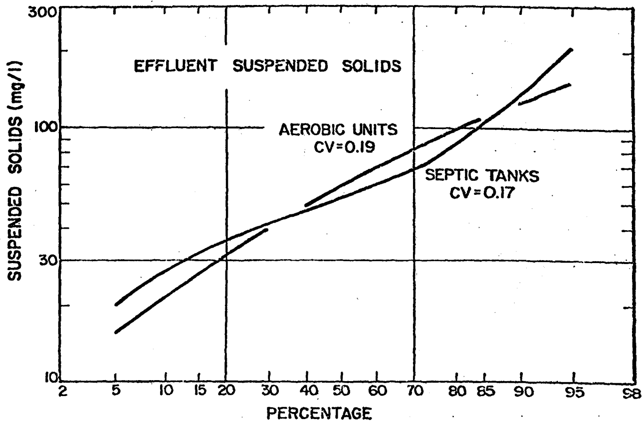
Figure III-D.2.b. Comparison of Septic Tank and Aerobic Unit Effluent Suspended Solids (Otis and Boyle, 1975)
