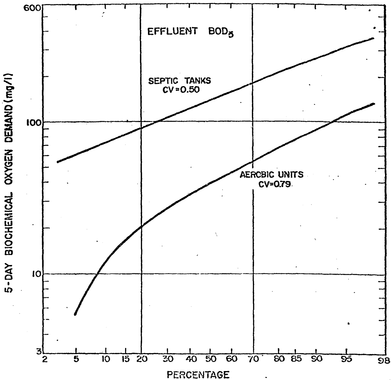
Figure III-D.2.a. Comparison of Septic Tank and Aerobic Effluent BOD 5 (Otis and Boyle, 1975)
