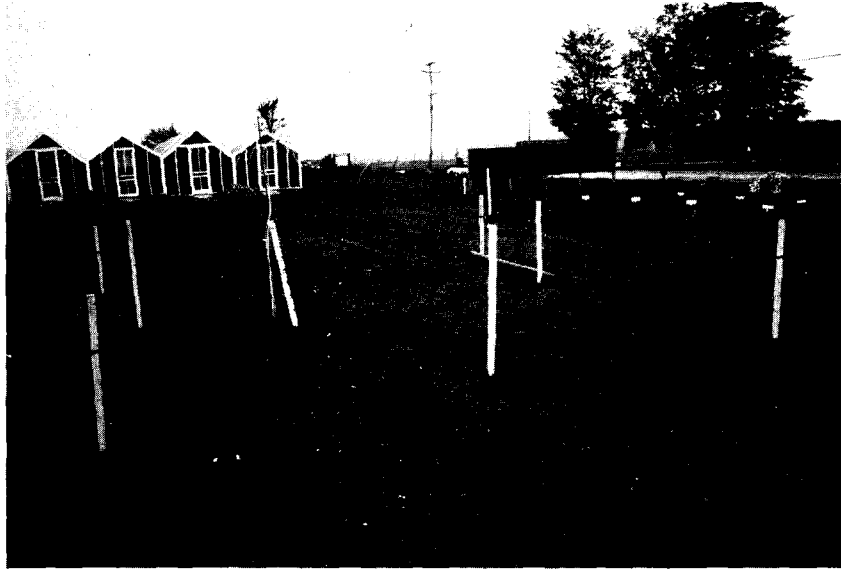
Fig. 2. Lay out the boundary of the fill system and the bed within the fill system. Take the necessary elevations in the fill system before plowing. These elevations are used to locate the bottom of the bed. Locate where the pipe from the pumping chamber will be placed. This pipe connects to the distribution system in the bed.
