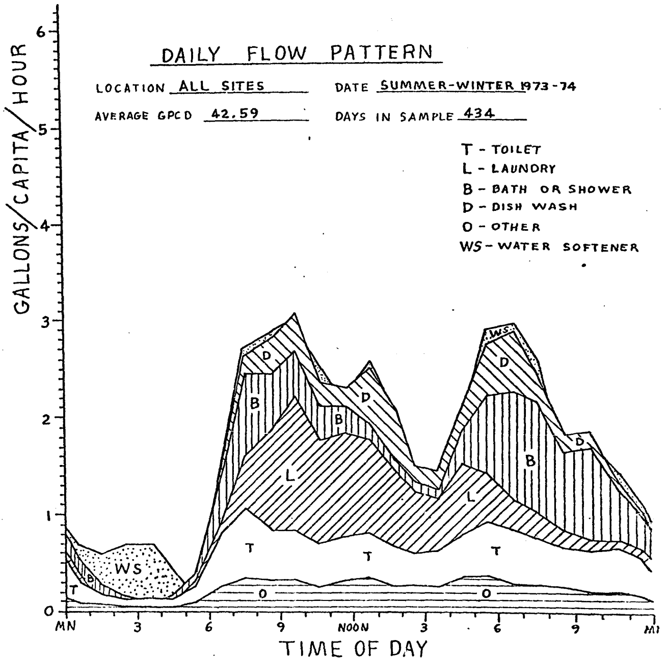
Figure III-A.1. Average Daily Flow Pattern From Eleven Rural Households (Witt, 1974)
