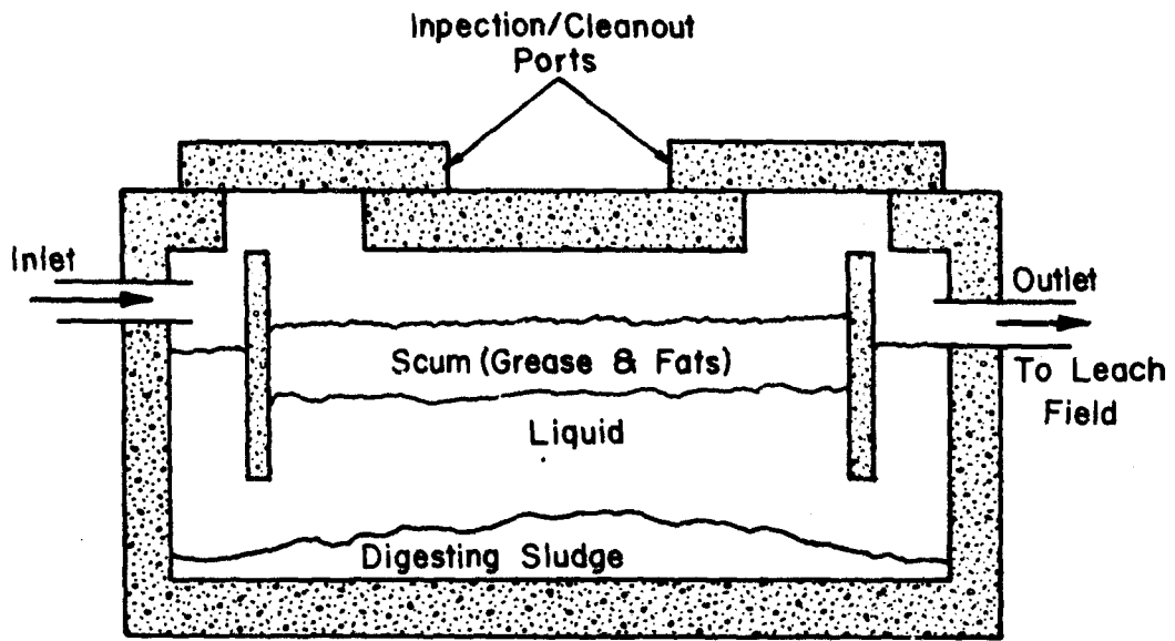
Figure 1-1. Septic Tank
