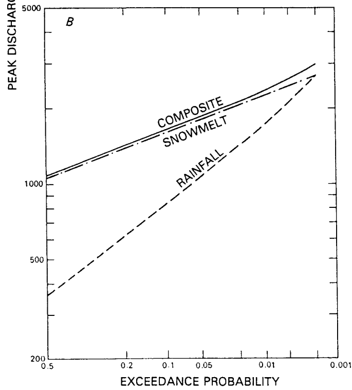
Figure 2.--Flood-frequency curves for Clear Creek near (A), Golden, Colorado (site 11), and (B), Lawson, Colorado (site 10).
