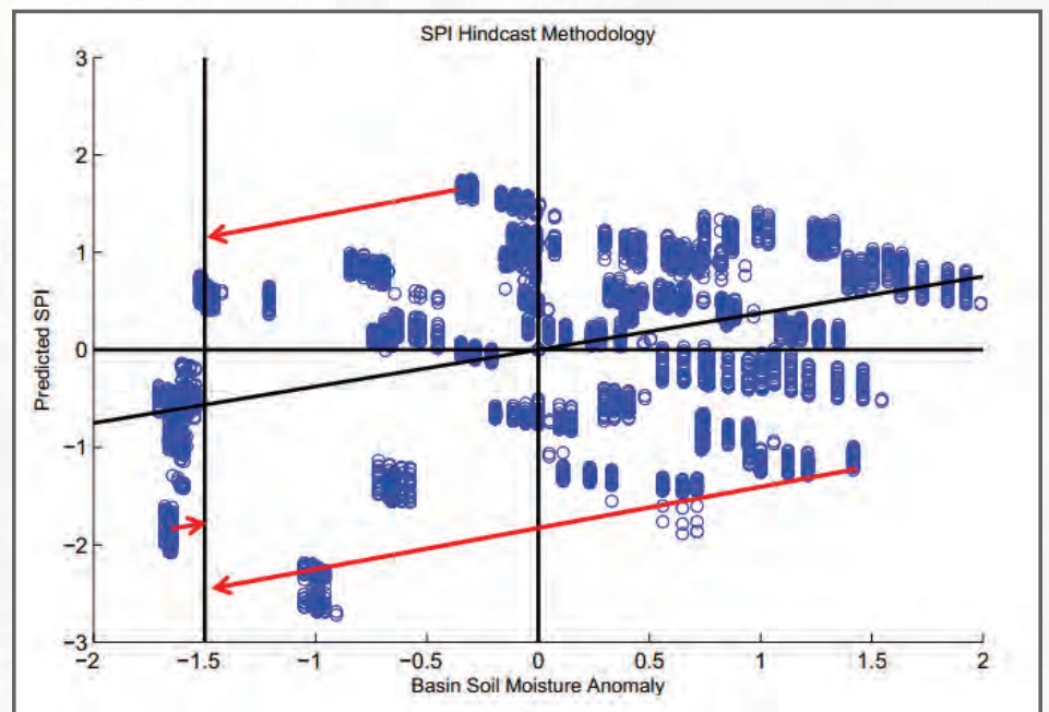
Figure 2. This scatterplot shows all of the data from the 1985-2014 period being considered for in the issuance of a precipitation hindcast for one of the nine subregions for the 90-day period beginning on May 1st, 2002. The black line at -1.5 illustrates the value of the 2002 subregion soil moisture anomaly, and the red arrows illustrate the method by which regressed SPIs are derived from actual SPIs.
