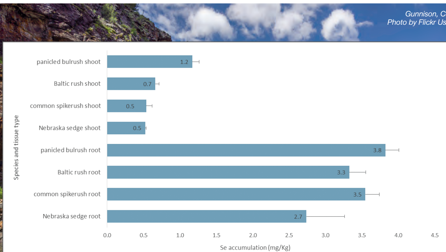
Figure 2. Average selenium concentration (mg/Kg) accumulated by the roots and shoots of four wetland plant species after a 4-month residence in a seleni-um rich gravel pit pond adjacent to the Colorado River in Mesa County, Colorado.
